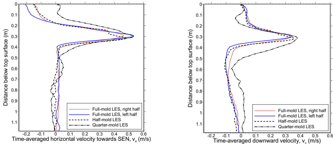
Figure 7. Time-averaged velocities along vertical line 152mm from SEN outlet, from LES.
