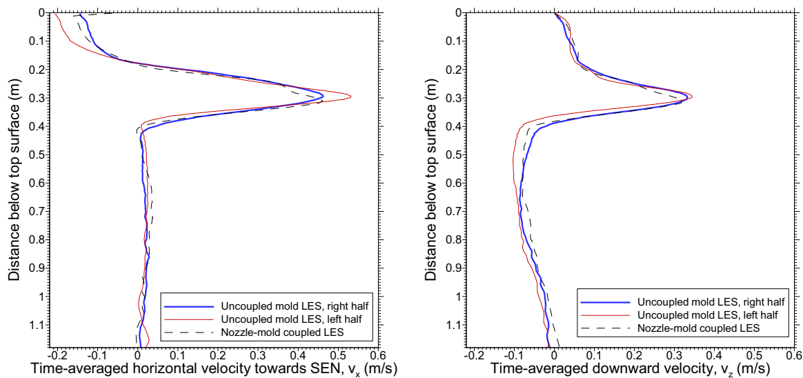
Figure 10. Comparison of time-averaged velocities obtained from nozzle-mold coupled and uncoupled mold simulation along a vertical line 152mm from the SEN outlet plane.
