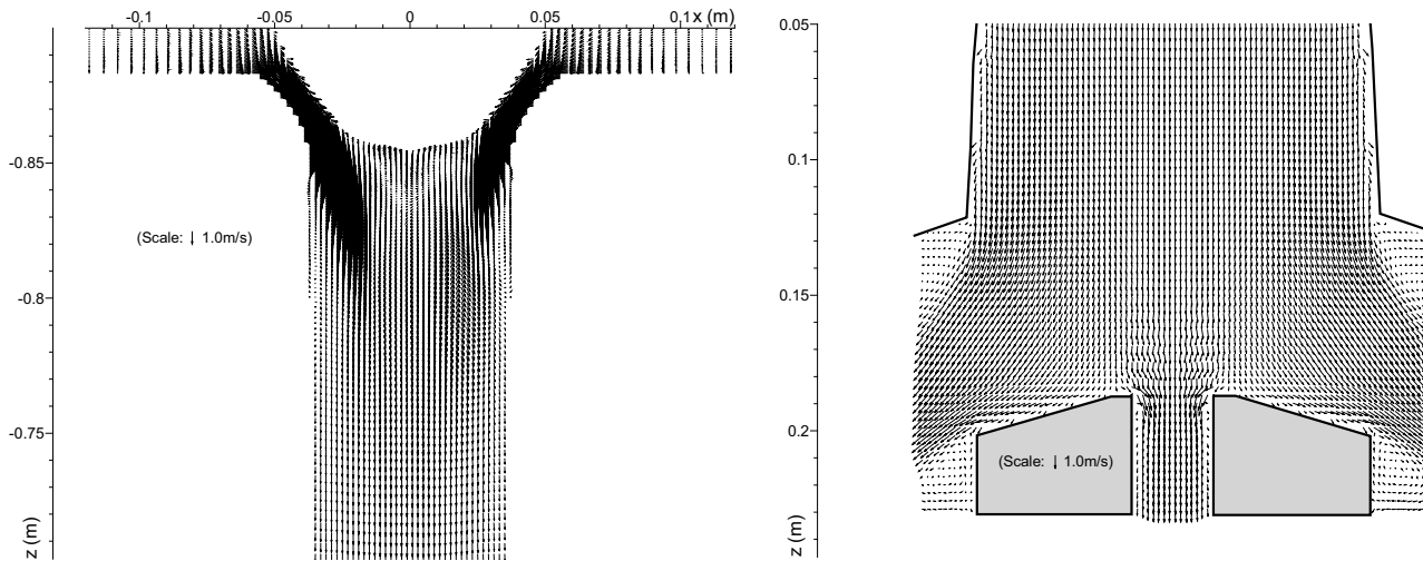
Figure 2. Computed flow velocities in nozzle near (a) stopper rod and (b) exit ports.
