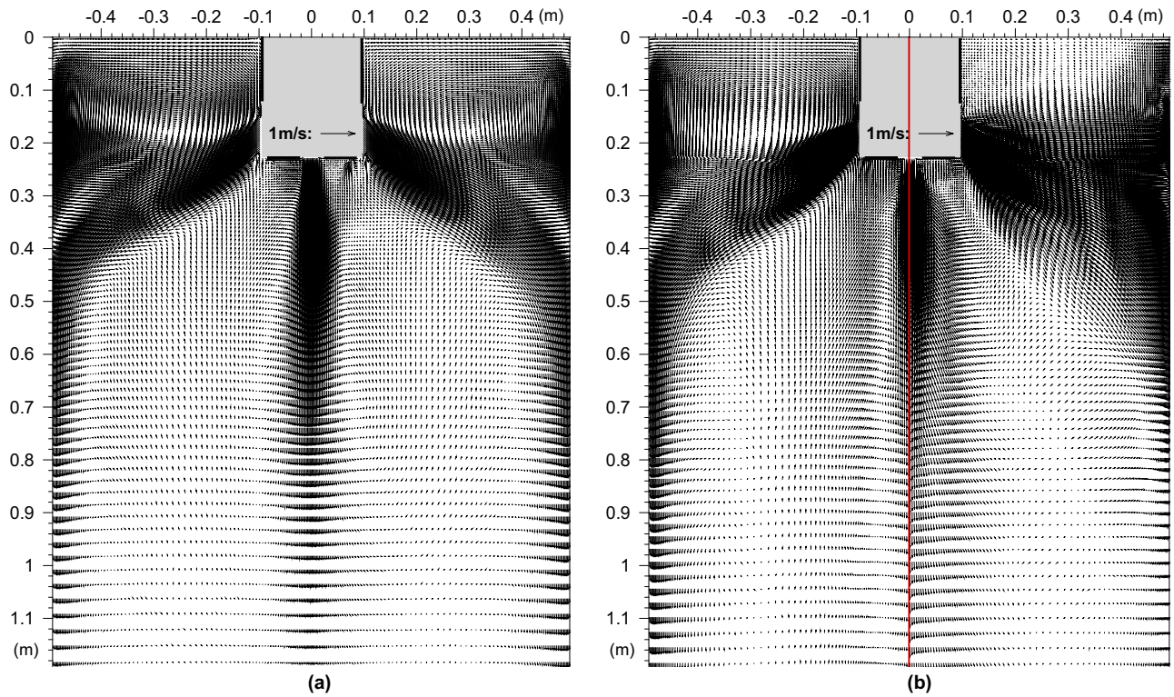
Figure 6. Effect of symmetry assumption on time-averaged velocity fields for simulation domains with (a) both halves (b) half (left) and quarter (right) of the mold region.
