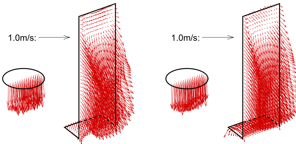
Figure 9. Comparison of time-averaged velocity vectors exiting nozzle ports obtained from (a) coupled simplified nozzle and (b) uncoupled complete nozzle simulations.
