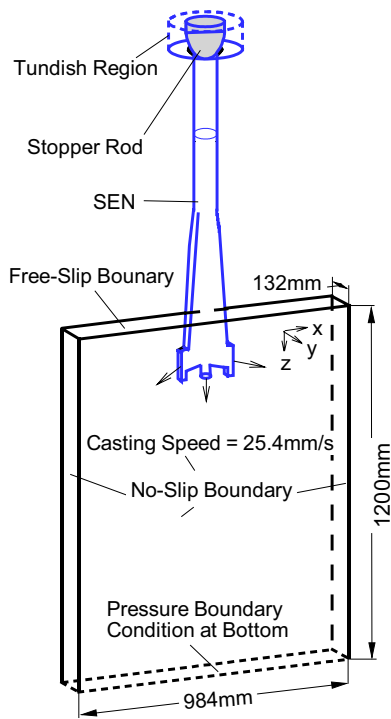
Figure 1. Schematic of the nozzle and mold domains.
