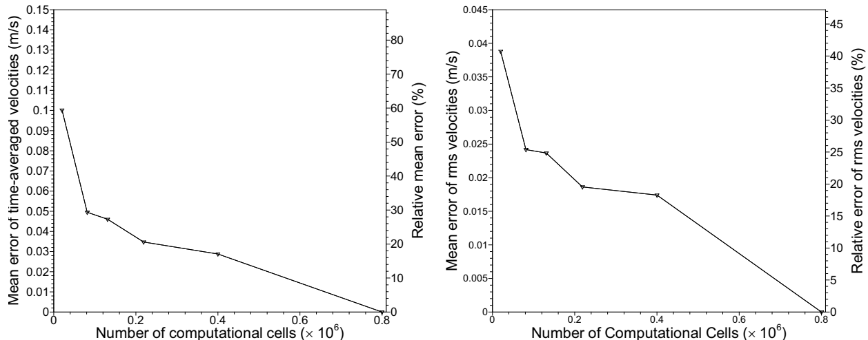
Figure 4. Effect of grid refinement on error in (a) time-averaged and (b) rms velocities.
